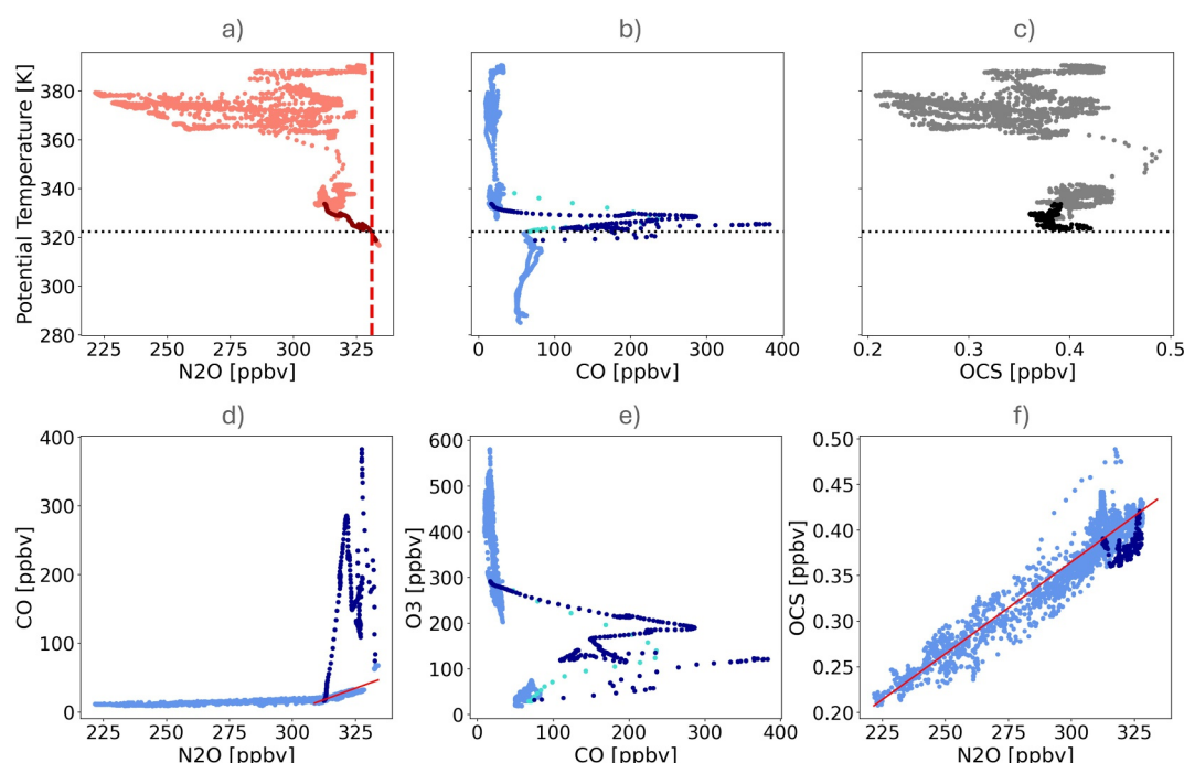
Figure 2. Vertical profiles as a function of potential temperature (a, b, c) and correlation plots of different species (d, e, f) for ST25. Biomass burning signatures are highlighted in dark colors, bright colors denote the rest of the flight. Cyan colors for CO in (b, e) indicate the second plume encounter during descent (no OCS/N 2 O data available). The black dotted line marks the tropopause identified from N 2 O threshold of 331.1 ppbv (red dashed line, a). The red line in (d, f) shows stratospheric background to detected plume.
