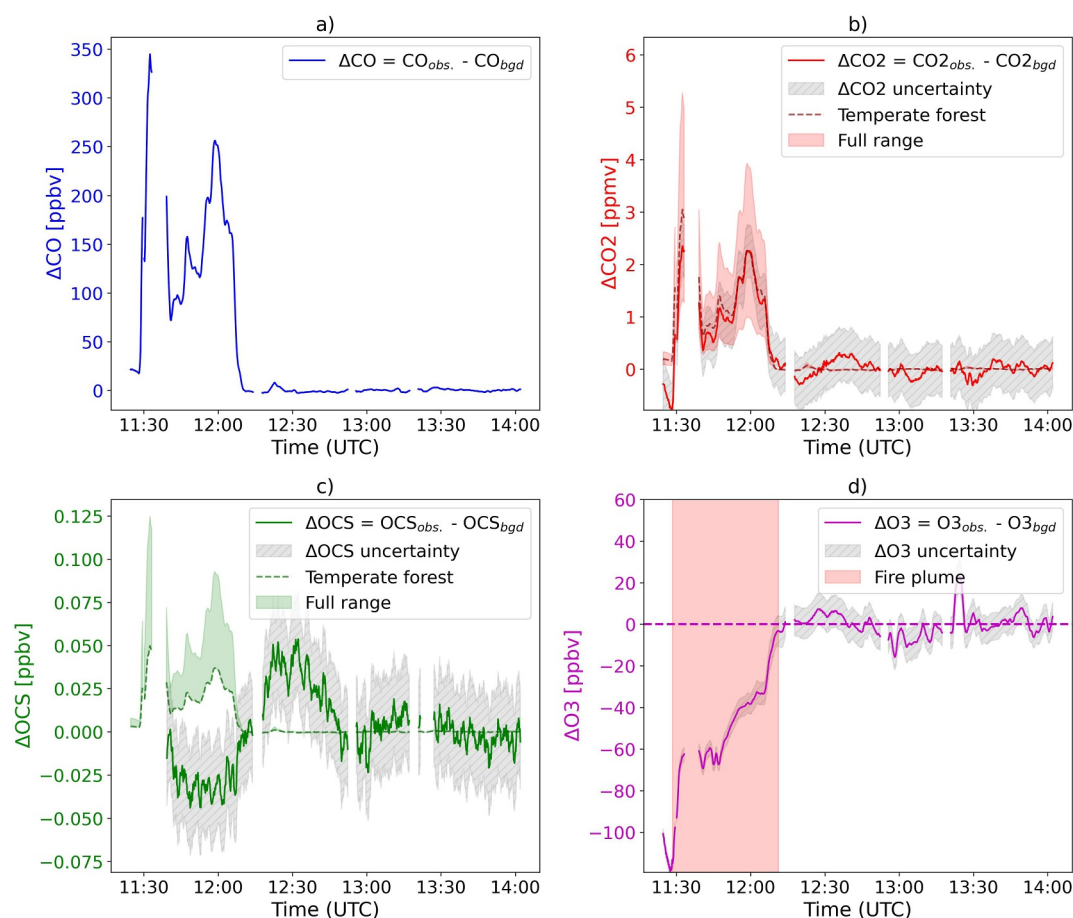
Figure 4. Enhancements in fire plume without background for CO, CO 2 , OCS and O 3 . Expected values for CO 2 and OCS related to CO were shown for the full range of vegetation types and for temperate forest (b, c). For O 3 , the red shaded area highlights the time range of the fire plume (d).
