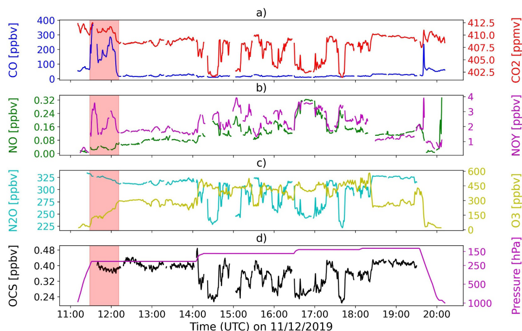
Figure 1. Time series of mixing ratios of CO, CO 2 , NO, NO y , N 2 O, O 3 and OCS, and pressure during ST25 (53.3°–70.3°S). The red shaded area indicates the identified biomass burning signatures shortly after the ascent.
