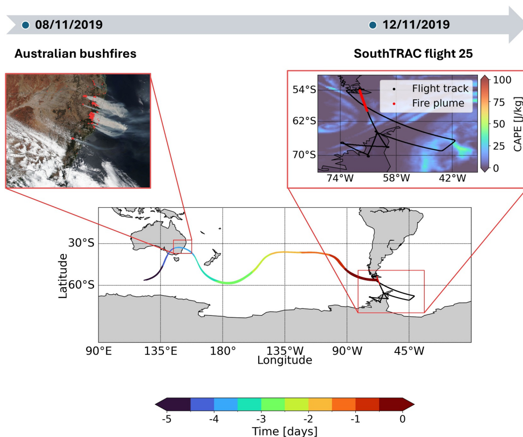
Figure 3. Lower panel: Backward trajectories started from the flight track (upper right) between 11:42–11:54 UTC during enhanced biomass burning tracer signatures of ST25. Satellite data from VIIRS at Suomi NPP observed on 8 November 2019 (upper left, NASA EOSDIS Worldview, 2025) indicate several biomass burning events marked with red dots in this region forming a fire plume moving eastwards.
